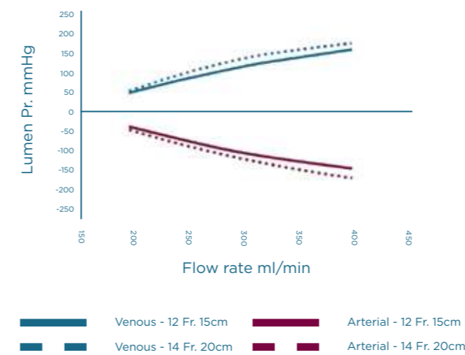
Kflow Epic Dual Lumen
